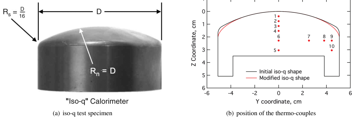
Figure 1: Definition of the geometry and dimensions of the iso-q test specimen. 5,6,8
