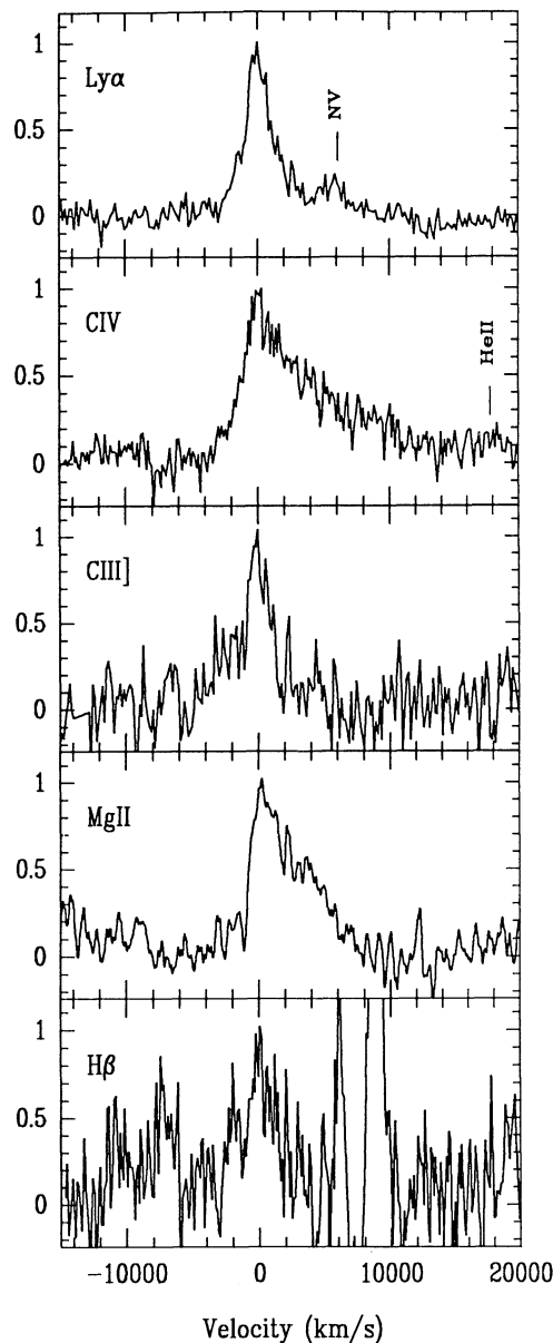
FIG. 2.—Observed emission line profiles in 3C 279, normalized to the line peak intensity. Note the very strong red wings of C IV \lambda 1549 and Mg II \lambda 2798 that are not present in the Ly \alpha and the C III] \lambda 1909 profiles. The zero of the velocity scale is defined by the redshift of [O III] \lambda 5007 .
