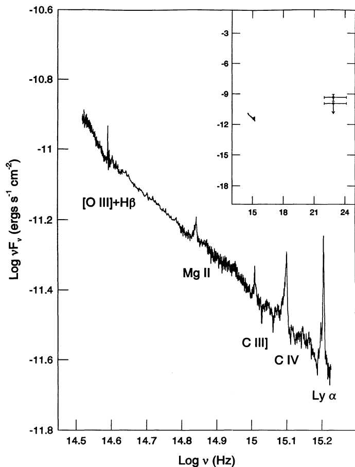
FIG. 1.—The 1992 April multiwavelength spectrum of 3C 279. The insert shows the combined optical-ultraviolet- \gamma -ray spectrum with the EGRET points from Kniffen et al. (1993), with the flux density uncertainty and the EGRET energy band indicated. A reddening correction corresponding to E(B-V) = 0.015 has been applied to the optical-ultraviolet data (Burstein & Heiles 1992).
